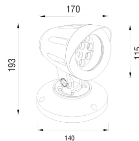
Đế ngồi/Surface-mounted
