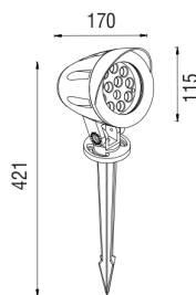
Cắm cỏ/Spike-mounted
