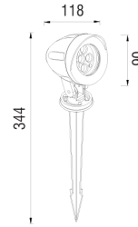
Cắm cỏ/Spike-mounted
