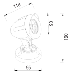
Đế ngồi/Surface-mounted
